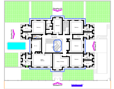
Second Floor Plan A = 398,75 m 2
