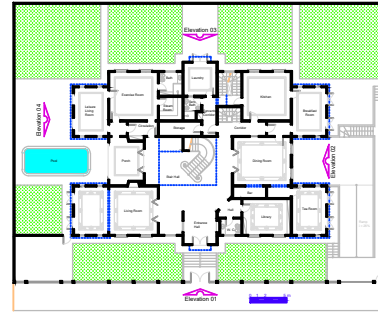
First Floor Plan A = 432,75 m 2
